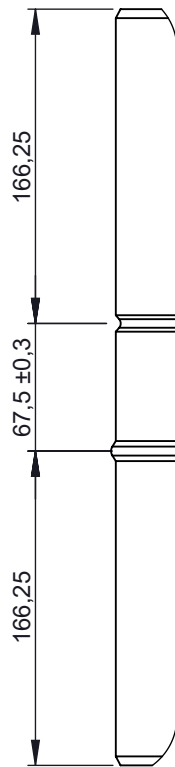
DETAIL C (1 : 4)
