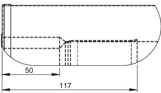
DETAIL A (1 : 2)
