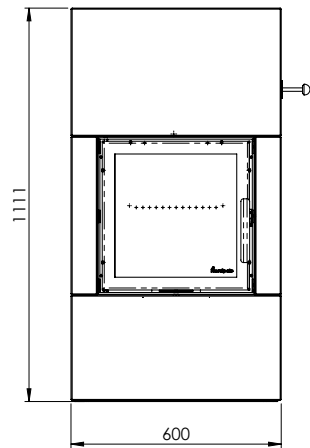
SALZBURG S - CONCRETE TOP PLATE = MM
