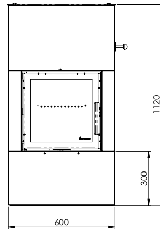
SALZBURG S - HOT TOP PLATE = MM
