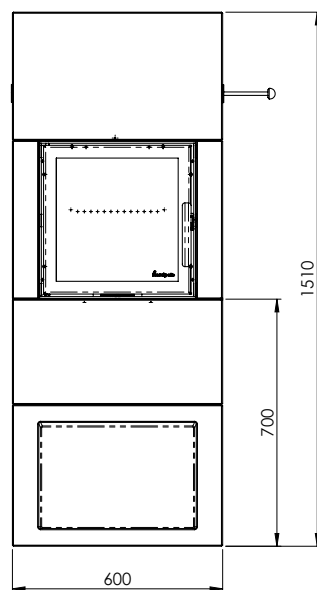
SALZBURG S - CONCRETE TOP PLATE/WOOD SHELF = MM
